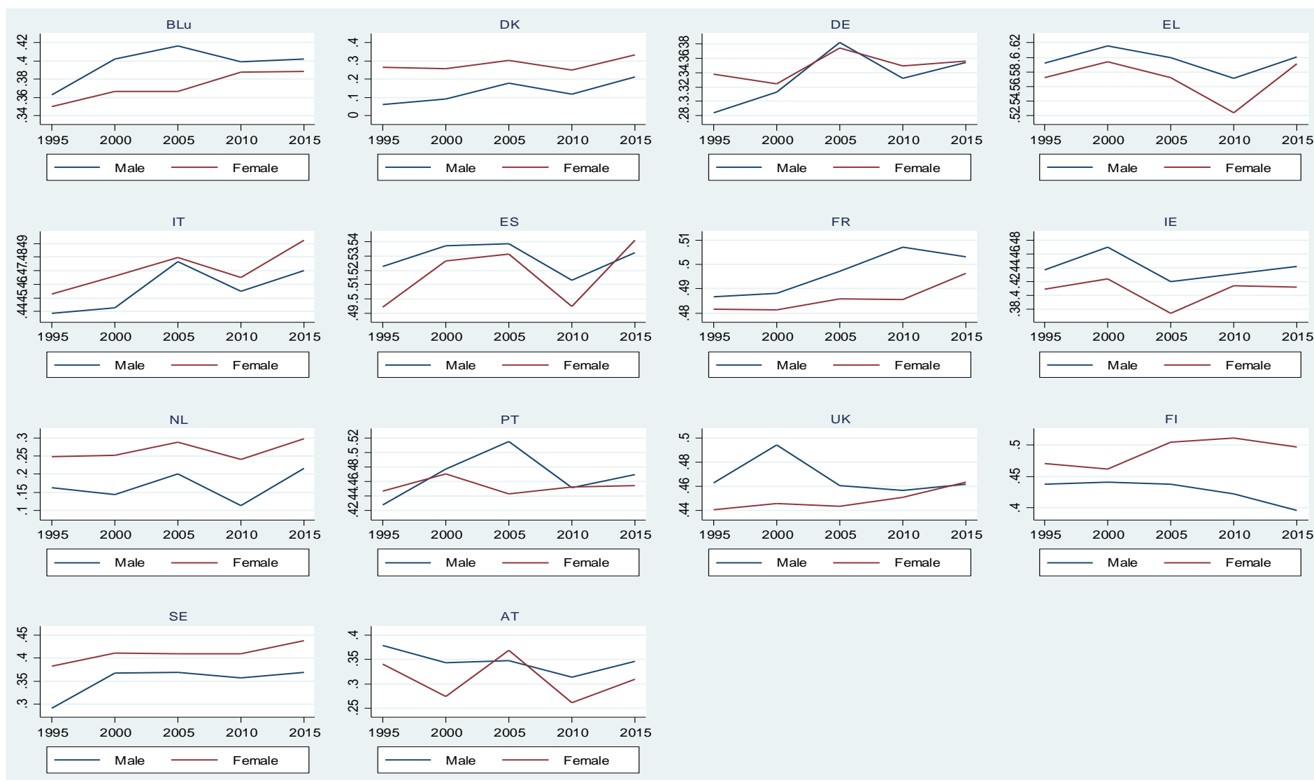
Figure A3. Average vulnerability per gender and by survey year for each country
