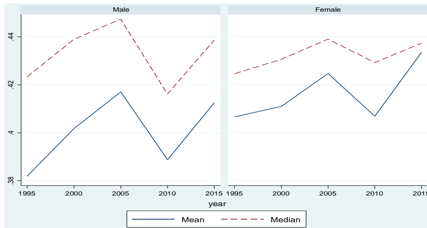
Figure 4. Average vulnerability by gender
