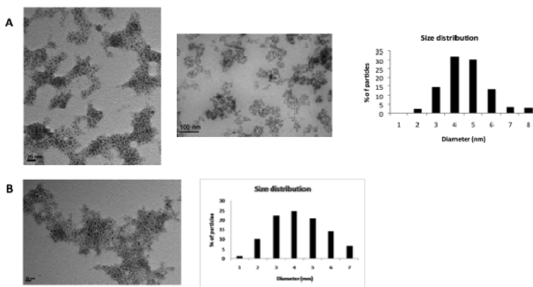
Figure 4. (A) Transmission Electron Microscopy images of synthesized bismuth NPs under sonication in batch and size distribution. (B) Transmission Electron Microscopy images of spherical synthesized bismuth NPs by flow chemistry coupled to sonication and size distribution.
