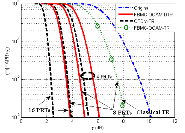
Fig. 3. CCDF of PAPR plot for FBMC-OQAM symbols with PAPR calculated over [T, 3T) with size of PRT set, R = \{4, 8, 16\} .
