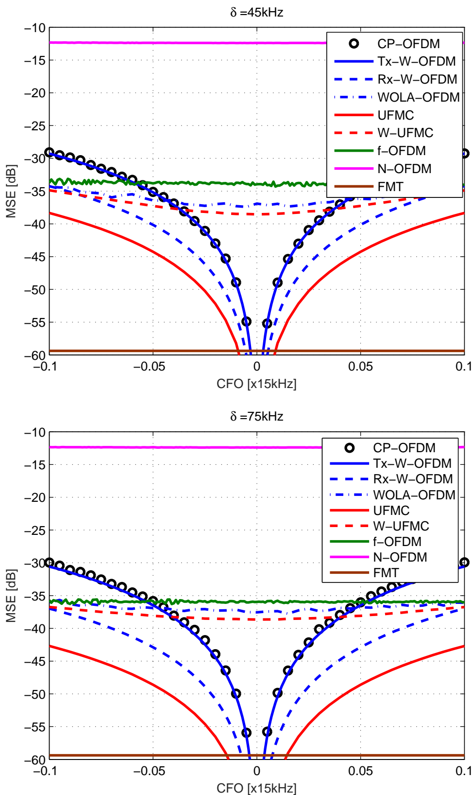
Figure 4-30: WFs with complex orthogonality: average MSE against CFO
