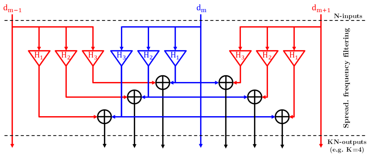
Figure 2-13: Frequency spread filtering
