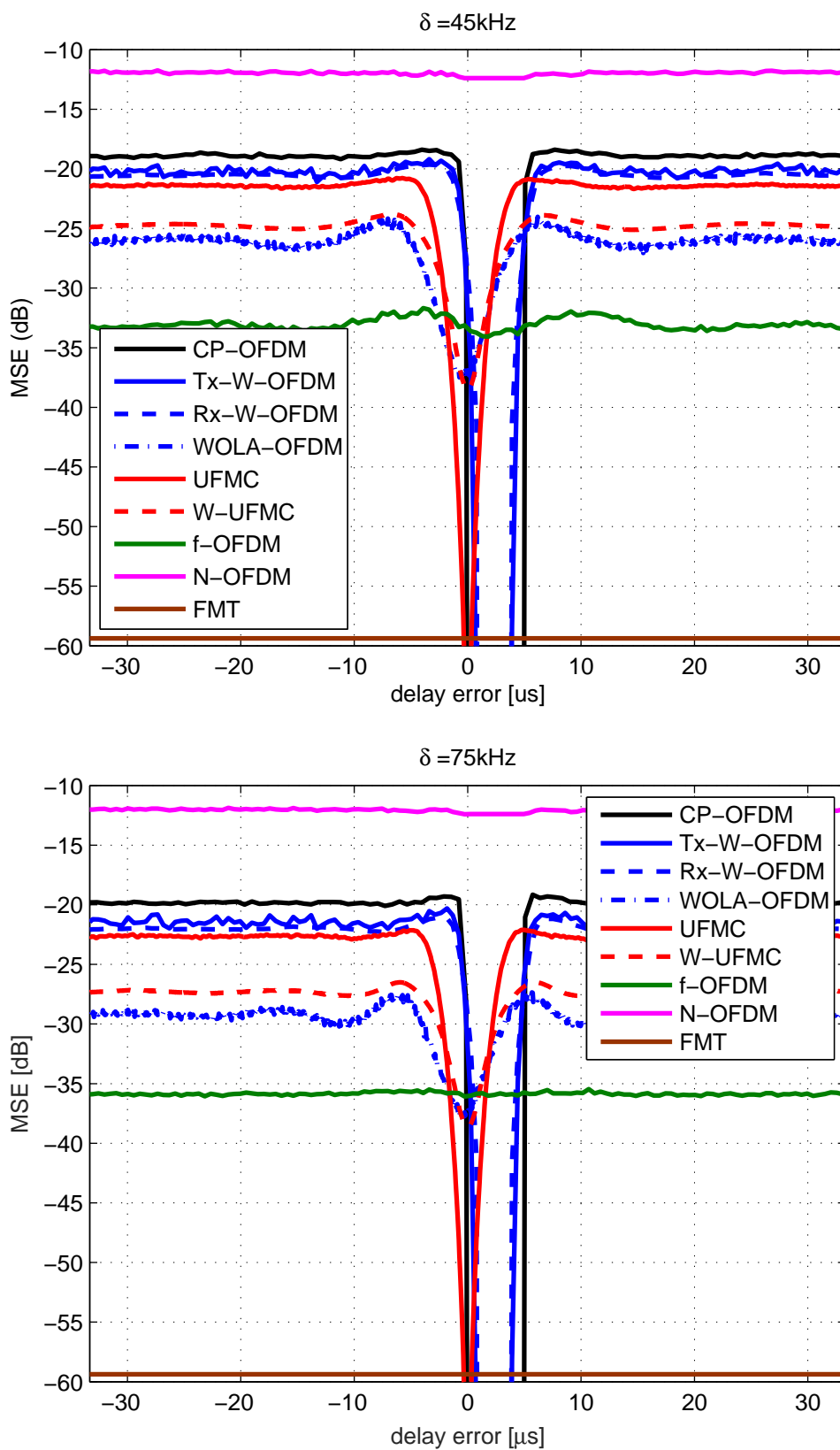
Figure 4-14: WFs with complex orthogonality: average MSE against timing offset
