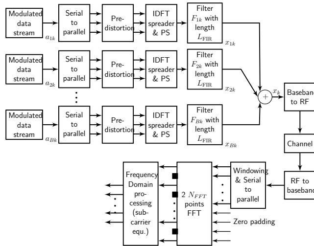
Figure 2-4: Block diagram of UFM C Tx and Rx processing [SW14b].
