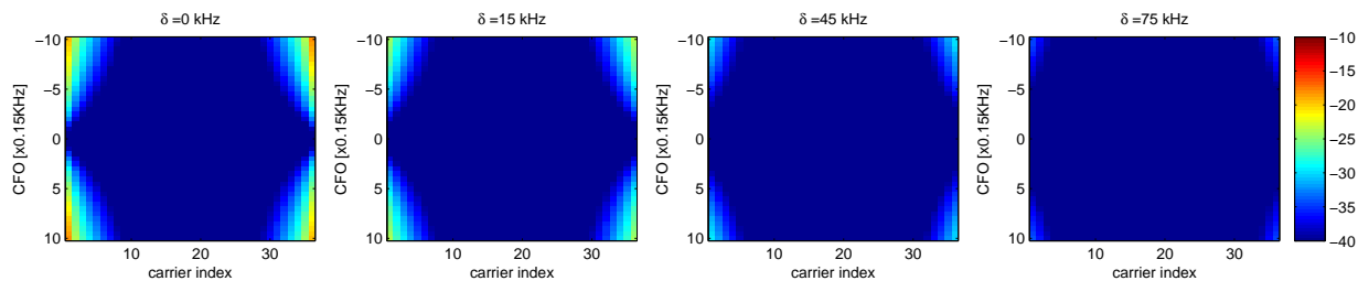
Figure 4-25: UFMC: per-subcarrier NMSE against CFO
