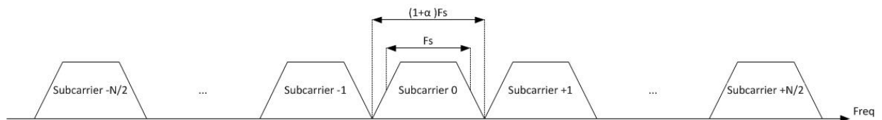
Figure 2-9: Frequency representation of FMT scheme.
