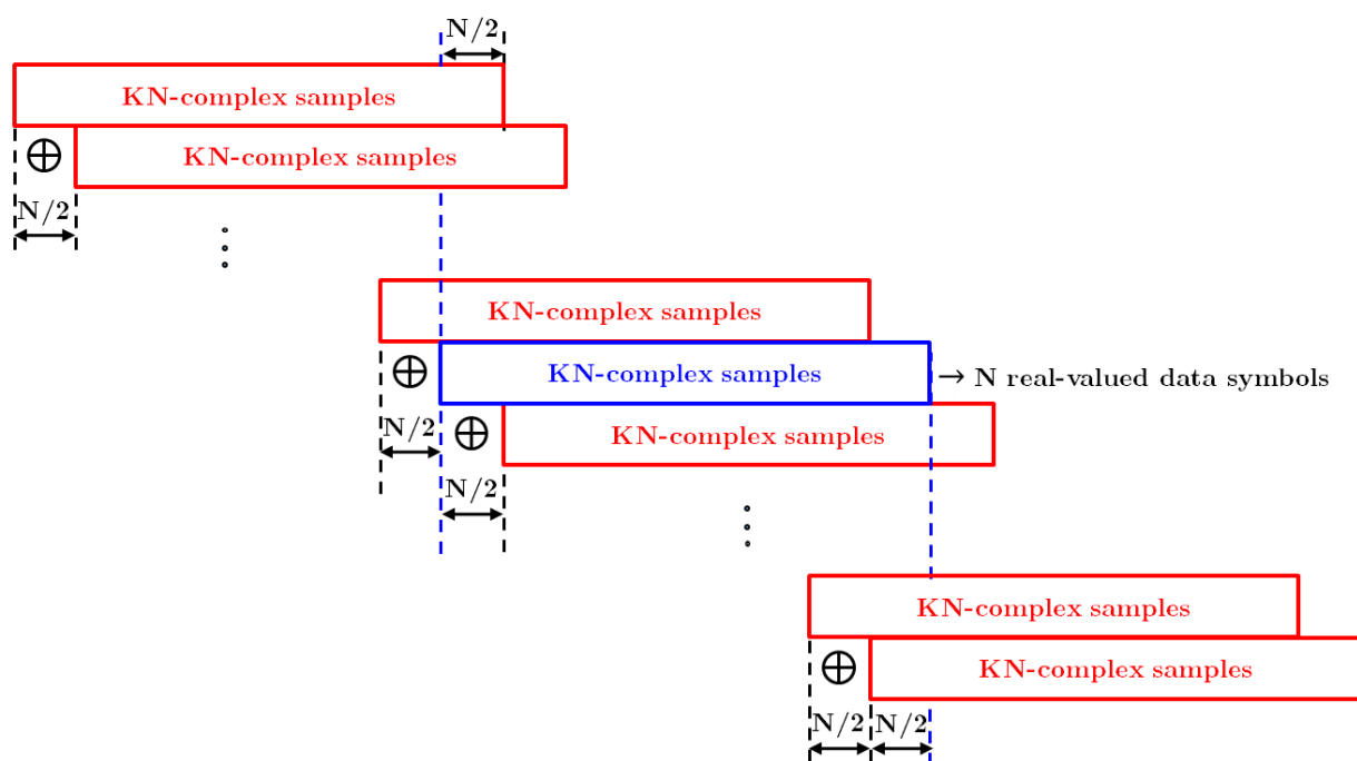
Figure 2-14: FBMC-OQAM transmitted signal
