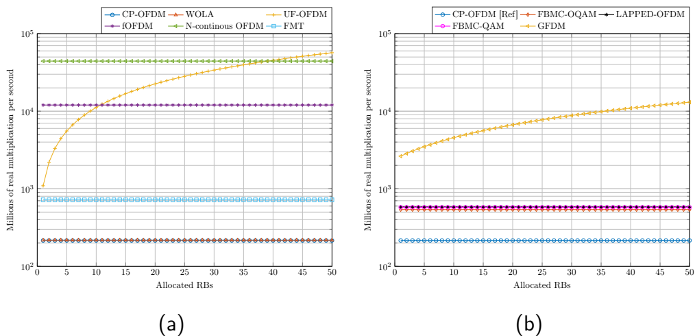
Figure 4-38: Tx complexity synthesis for waveforms satisfying the complex orthogonality (a) and for waveforms that do not satisfy the complex orthogonality (b)
