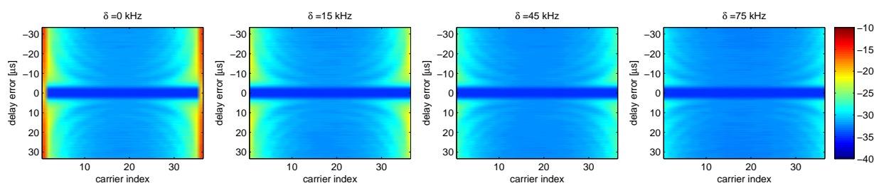
Figure 4-20: MF-GFDM w. IC: per-subcarrier NMSE against timing offset
