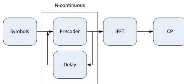
Figure 2-8: Block diagram of N-continuous OFDM scheme.
