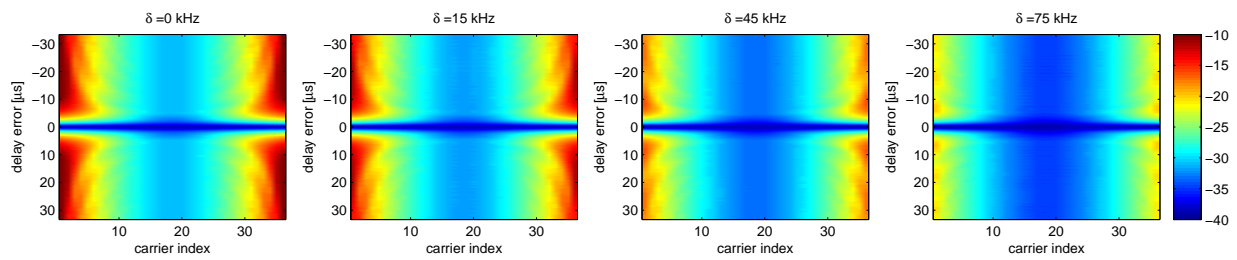
Figure 4-10: W-U-FMC: per-subcarrier NMSE against timing offset
