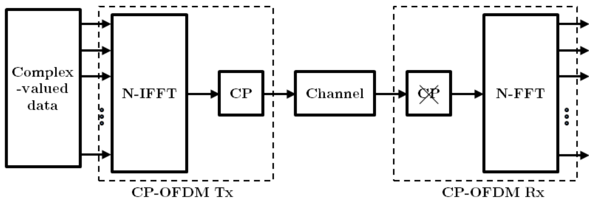
Figure 2-1: CP-OFDM transceiver
