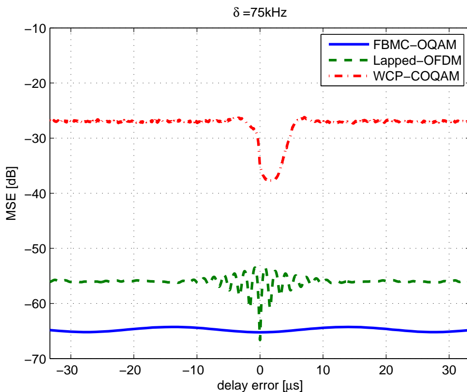
Figure 4-18: WFs with real orthogonality: average MSE against timing offset
