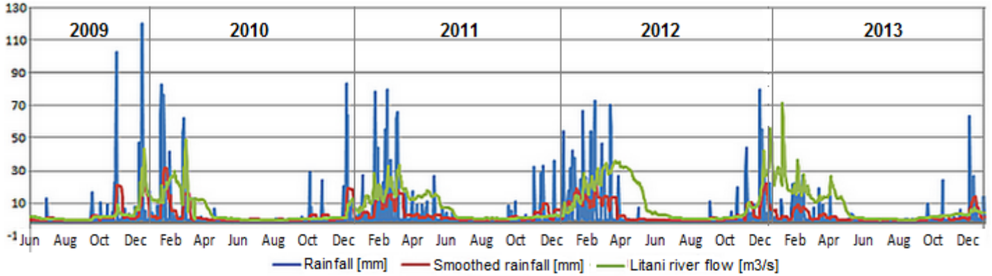
Figure 10. Daily river flow ( m^3/s ), rainfall ( mm ) and filtered rainfall ( mm ) starting 01 Jun. 2009 till 31 Dec. 2013.
