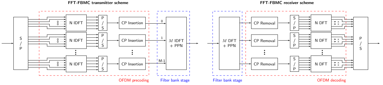
Figure 1. FFT-FBMC transmitter and receiver schemes
