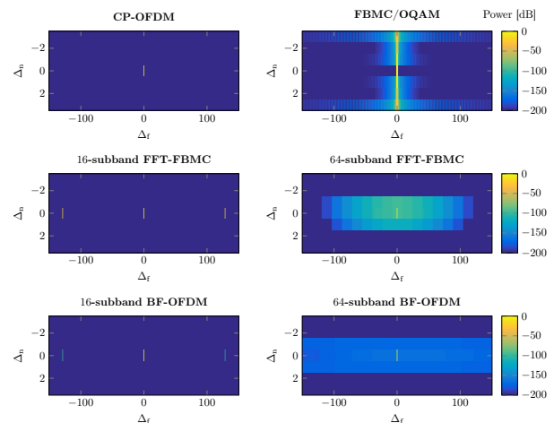
Figure 4. Transmultiplexer response of the considered waveforms where \Delta_f denote the subcarrier offset and \Delta_n the time instant offset.
