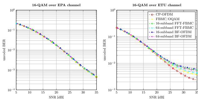
Figure 6. Uncoded BER for SISO 16-QAM over 5-Hz EPA and 300-Hz ETU channels.
