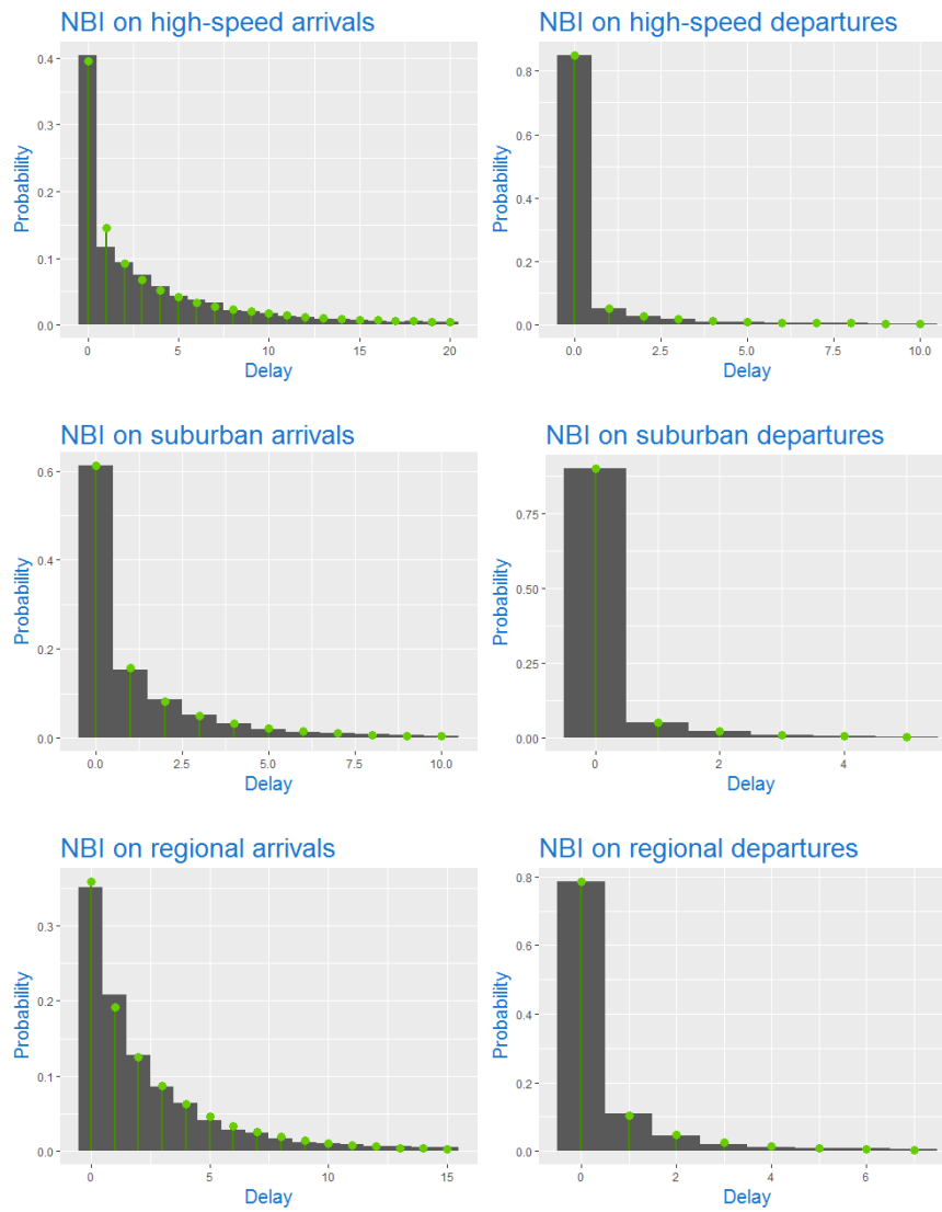
Figure 3: Negative binomial
