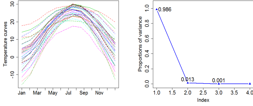
Figure 3: The temperature curves of 34 cities in training set (left), the eigenvalues of the sample covariance function (right).
