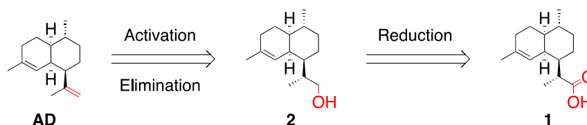
Scheme 2. Formation of amorpha-4,11-diene, AD , from dihydroartemisinic acid, 1 .
