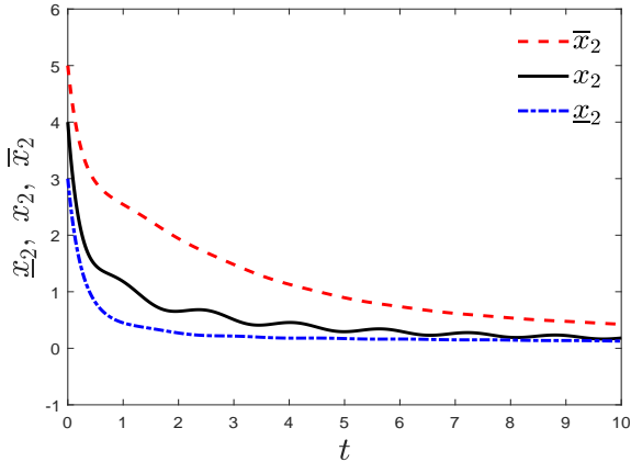
Fig. 1. The interval [\underline{x}_2, \bar{x}_2] estimated by the observer (5) with (24) and (26) for plant (1) given by (23) with initial condition (27) and disturbance (28).
