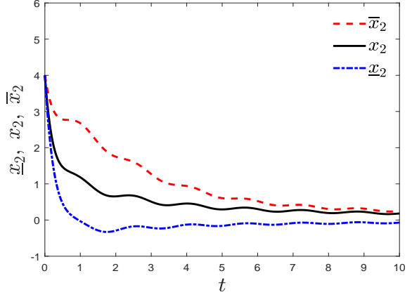
Fig. 4. The interval [x_2, \bar{x}_2] estimated by the observer (5) with (24) and (31) for plant (1) given by (23) with initial condition (29) and disturbance (30).
