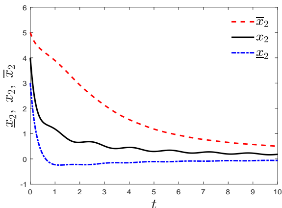
Fig. 3. The interval [\underline{x}_2, \bar{x}_2] estimated by the observer (5) with (24) and (31) for plant (1) given by (23) with initial condition (27) and disturbance (28).
