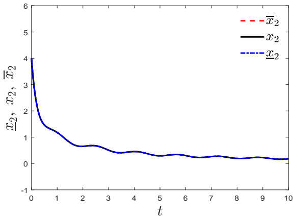
Fig. 2. The interval [\underline{x}_2, \bar{x}_2] estimated by the observer (5) with (24) and (26) for plant (1) given by (23) with initial condition (29) and disturbance (30); The three lines completely overlap.
