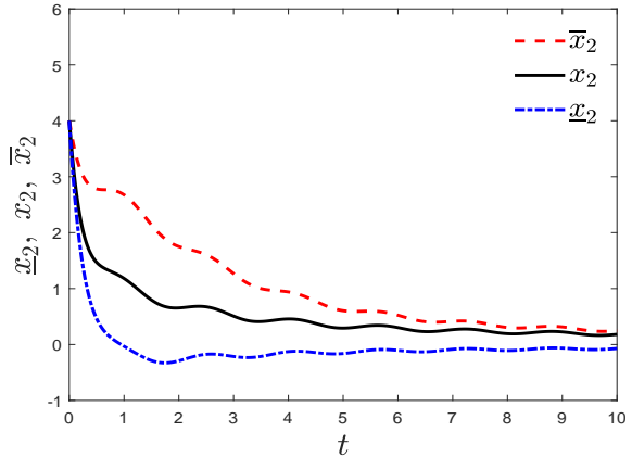
Fig. 4. The interval [\underline{x}_2, \bar{x}_2] estimated by the observer (5) with (24) and (31) for plant (1) given by (23) with initial condition (29) and disturbance (30).
