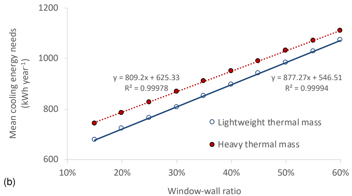
Fig. 14. Mean cooling energy needs as given by dynamic simulation versus window-wall ratio: (a) Helsinki and (b) Athens.
