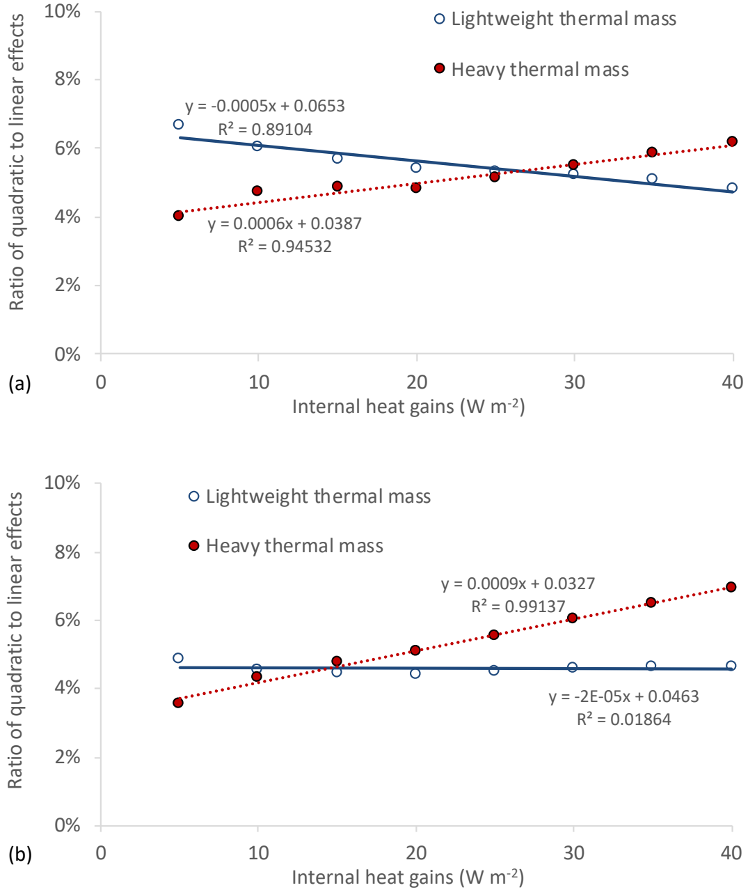
Fig. 11. Ratio of quadratic to linear effects for Athens versus internal heat gains: (a) absolute value and (b) root mean square.
