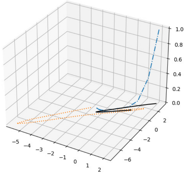
Figure 4: Simulation for (48). Here \alpha = 0.4 and \Delta t = 0.1 , the dotted curve is the value of the velocity v_n . The solid curve describes the coordinates of u_n . The dash-dotted curve corresponds to the sequence (u_n, F(u_n, v_n)) .
