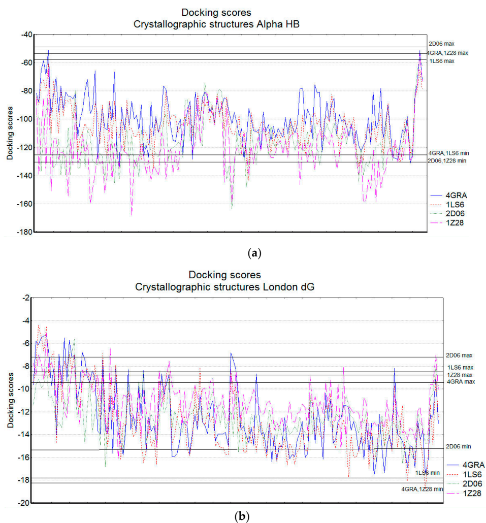
Figure 11. Docking scores of the selected natural products (159 compounds) in the crystallographic enzyme structures using: (a) Alpha HB scoring function; (b) London dG scoring function. The lines represent the levels of the minimal and maximal scores obtained for the group of natural SULT ligands.
