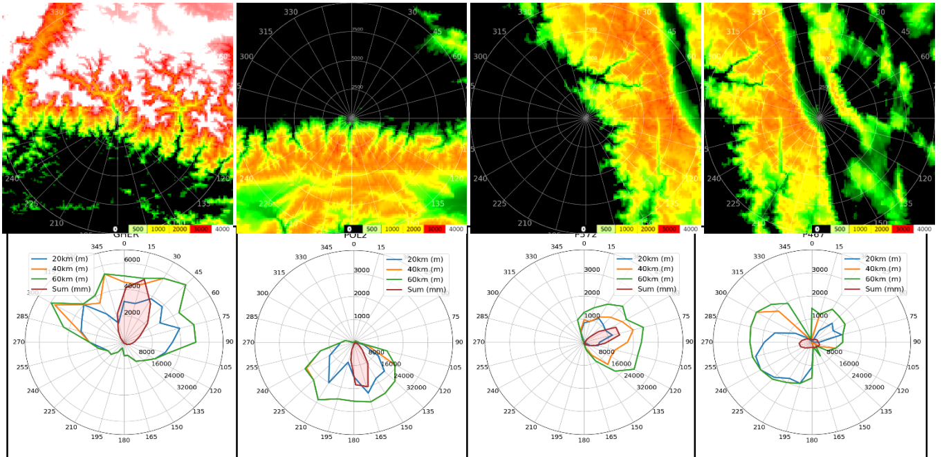
Fig. 6. Relative location of mountains from the station (top charts). Gradients and relief curves (bottom radar charts centred on station location) for class 1 stations: GHER (Himalaya), POL2 (Nepal), P572 and P467 (California near Sierra Nevada). Red curve (filled with pink) represents the gradient and the other curves represent the relief at different distances from the station: blue for 20 km, orange for 40 km and green for 60 km. Y axis legend corresponds to the elevation in m. (scale is different for GHER as it is situated in Himalaya, with height difference up to 6 km). Other axis legend (at 135° azimuth) corresponds to the sum of gradient.
