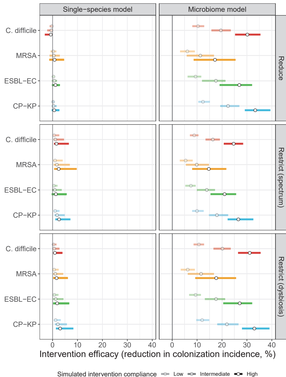
Appendix 1—figure 17. Intervention efficacy for three considered types of antibiotic stewardship: (i) reducing overall antibiotic prescribing, (ii) restricting broad-spectrum antibiotics in favour of narrow-spectrum antibiotics, and (iii) restricting antibiotics categorized as inducing microbiome dysbiosis at high or very high rates in favour of those that induce dysbiosis at medium or low rates. In microbiome simulations, restricting antibiotics that induce dysbiosis at a high rate was approximately as effective as reducing overall antibiotic prescribing. In single-species simulations, all stewardship interventions were of limited to negligible efficacy. Points correspond to medians, and bars to 95% uncertainty intervals across 10,000 Monte Carlo simulations.
