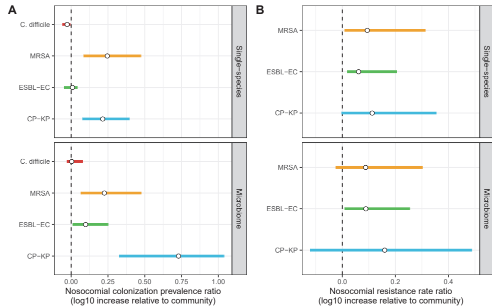
Appendix 1—figure 12. Change in ARB colonization outcomes in the hospital relative to the community ( \log_{10} scale), comparing single-species and microbiome simulations. ( A ) The ratio of colonization prevalence among hospital patients relative to baseline colonization prevalence in the community. ( B ) The ratio of resistance rates in the hospital relative to baseline resistance rates in the community. Points represent medians and error bars represent 95% uncertainty intervals across 10,000 Monte Carlo simulations.
