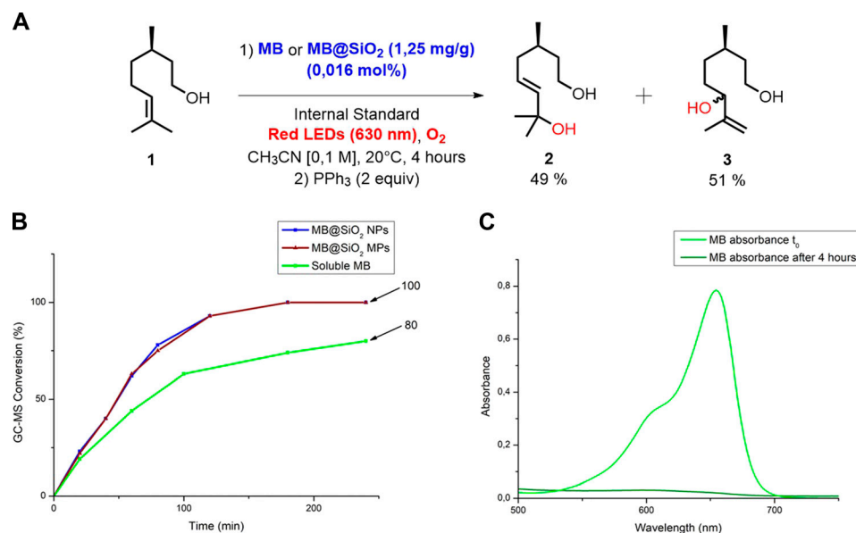
FIGURE 2 | (A) Photooxidation of 1 using MB or MB/SiO 2 as a PC under red light irradiation (630 nm) (B) Monitoring of the conversion of 1 to 2 and 3 in a batch reactor, in function of time by GC-MS analysis (Internal Standard = 1,3-dimethoxybenzene). The ratio between 2 and 3 is measured by 1 H NMR spectroscopy. (C) Absorption spectra of the homogeneous reaction media obtained at t 0 and after 4 h of reaction.
