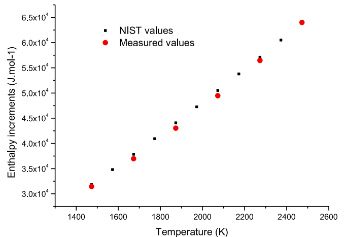
Fig. 8. Comparison of the measured enthalpy increments of tungsten with NIST values.
