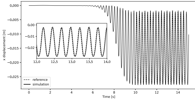
(a) Displacement of point A in x -direction
