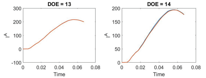
Fig. 14. Predicted temporal evolution (red) versus real temporal evolution (blue) for an Abdomen point inside the training set (left) and outside the training set (right).
