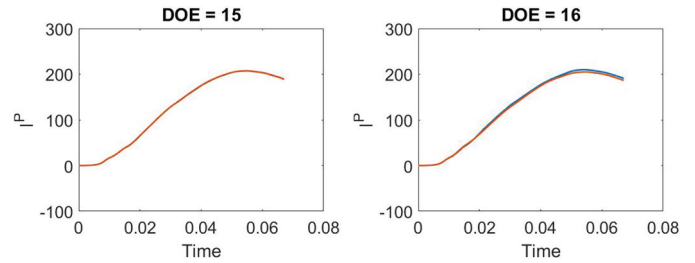
Fig. 15. Predicted temporal evolution (red) versus real temporal evolution (blue) for a Pelvis point inside the training set (left) and outside the training set (right).
