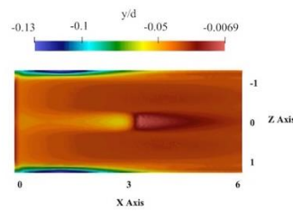
Fig. 4. Computed contours of bed elevation at t = 3 min, the turbine is located at x = 3 m.
