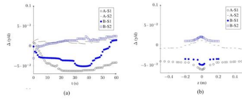
Fig. 18. Difference in dimensionless bed elevation between the baseline and turbine results at S_1 and S_2 , the erosion is represented as negative values. (a): temporal evolution of (\Delta y/d) , and (b): spatial evolution of \Delta y/d laterally in the cross section at time t = 40 s.
