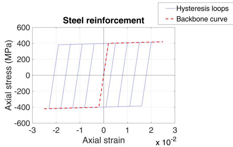
Figure 7. Steel reinforcement axial stress-strain curve
