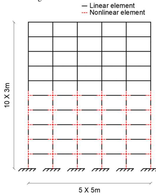
Figure 6. Position of nonlinear elements in RC frame
