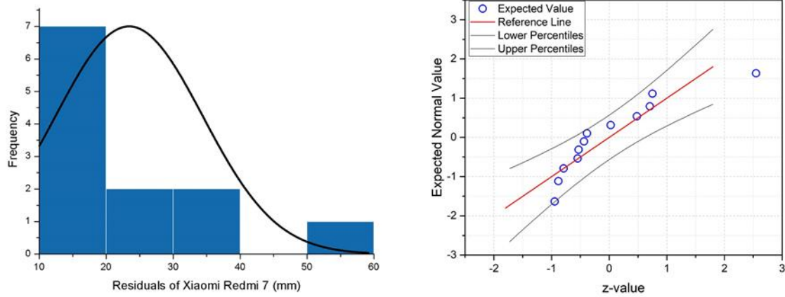
Figure 9. Histogram and Q-Q plot of photogrammetry using Redmi phone and Total station residuals with normal distribution (before outliers removing)
