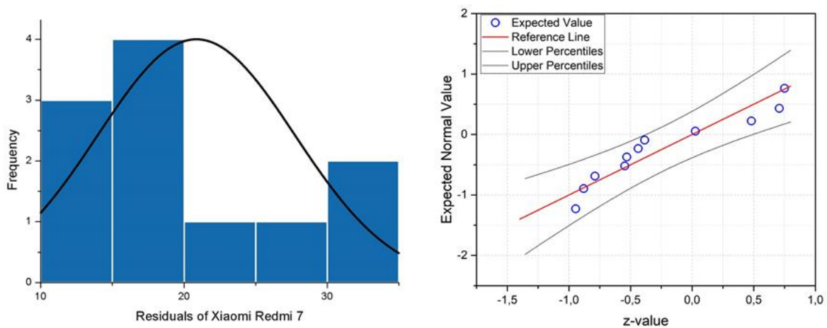
Figure 10. Histogram and Q-Q plot of photogrammetry using Redmi phone and Total station residuals with the normal distribution (after outliers removing)
