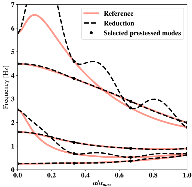
Fig. 9. Evolution of frequencies as a function of load parameter with 10 POD modes and 20 prestress modes.
