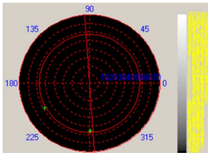
Figure 7. Measurement done using the EZ-Contrast. The studied sample is a physically eroded PMMA. The specular peak is located at the intersection of the circular continuous line and the diagonal line and is very narrow. This measurement shows the high level of gloss of our samples.
