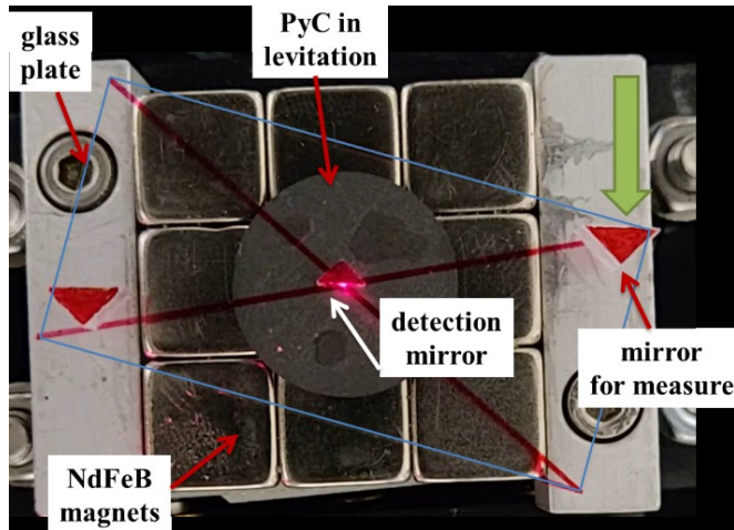
Fig. 4. Picture of the sensitive part of the LPM with NdFeB magnets, detection mirror and mirror for measure the optical power of the laser.
