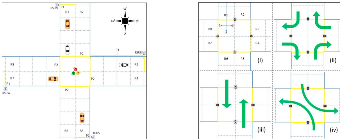
(a) IIMA on a four-way single-lane intersection
