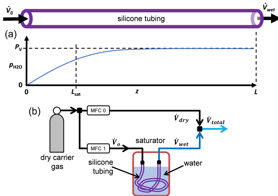
Figure 1. (a) Dry gas that enters a permeable tube immersed in water becomes more humid. The exiting gas is saturated if the tube is much longer than the characteristic length L_{sat} . (b) The humidity generator combines a stream of humid gas with a stream of dry gas.
