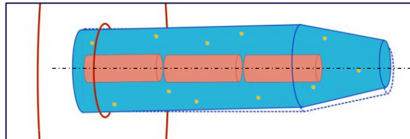
Installation of the misaligned cryostat inside the experiment so the FFQ are aligned
