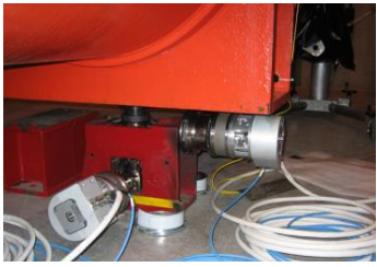
LHC / HL-LHC full remote alignment system for the Low-β quadrupoles
