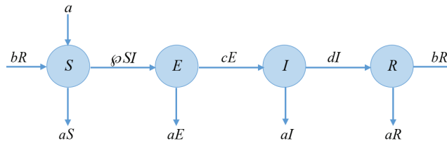
Figure 1. Block diagram for SEIR model.
