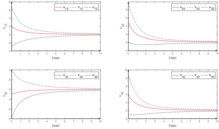
Figure 4. The bounds of the second state for the four-agents.
