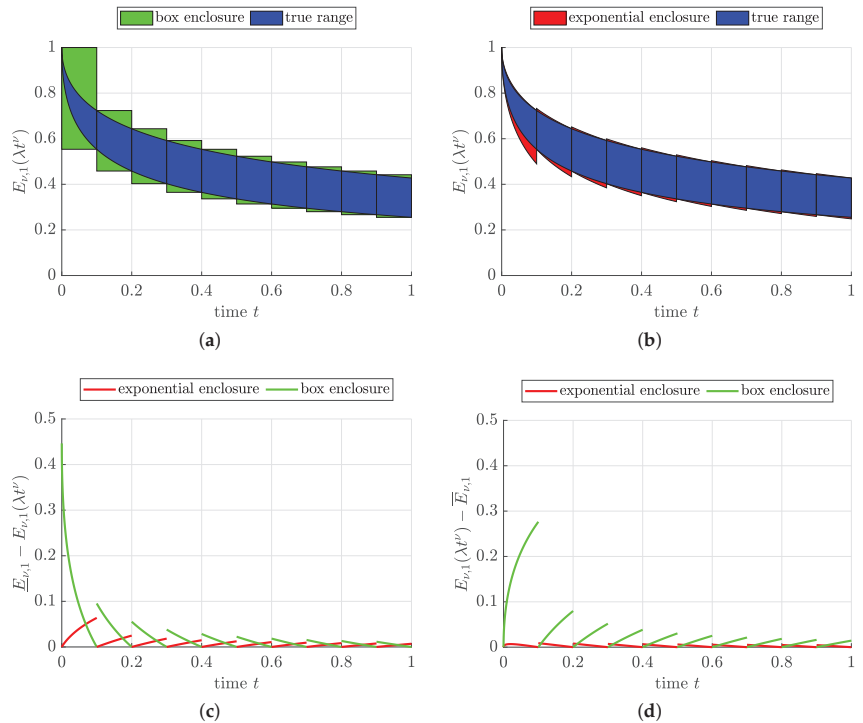
Figure 1. Comparison between box-type and exponential enclosures of the Mittag-Leffler function E_{\nu,1}(\lambda t^\nu) with \nu = 0.5 for t \in [0; 1] , t = k \cdot 0.1 , \bar{t} = (k + 1) \cdot 0.1 , k \in \{0, 1, \dots, 9\} , and \lambda \in [-2; -1] : (a) Box-type enclosure of the Mittag-Leffler function; (b) Exponential enclosure of the Mittag-Leffler function; (c) Overestimation of the lower enclosure bound; (d) Overestimation of the upper enclosure bound.
