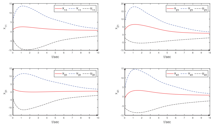
Figure 3. The bounds of the first state for the four-agents.
