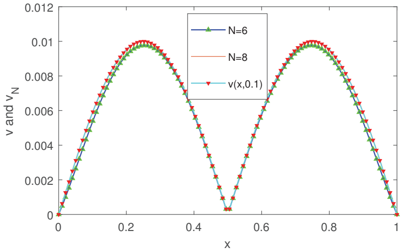
Figure 5. Plot of the numerical solutions for different values of \mathcal{N} at t = 0.1 for Example 2.
