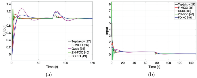
Figure 11. (a) Output signals for FO-PID control of lag-dominant process (b) Input signals for FO-PID control of lag-dominant process. Controllers tuned according to [26,27,36,40,49].
