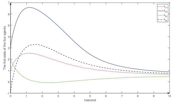
Figure 1. The first state of the four-agents.
