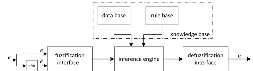
Figure 2. Block diagram of two-dimensional FLC.
