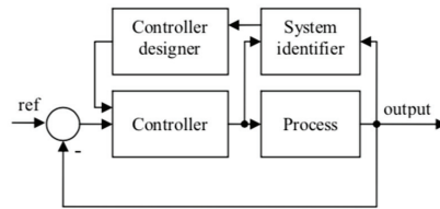
Figure 20. The self-tuning FO-PI controller.
