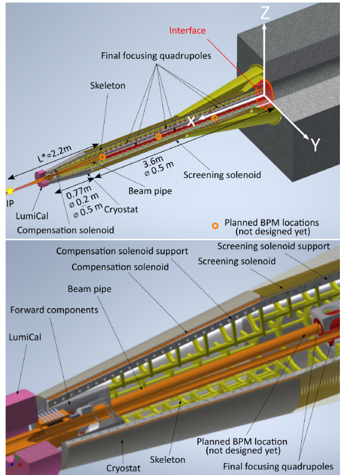
Figure 1. Inner components, original assembly. On the top picture, a general view of the assembly and the coordinate system associated to the plate. The second picture is zoomed in order to see the different elements, from the inside out: the beam pipe (orange), the final focusing quadrupoles (red), the skeleton (yellow), the support and cooling structure for the solenoids (gray), the screening and compensation solenoids (orange) and the thin cryostat (gray). The free length ( L^* ) corresponds to the distance between the IP and the face of the closest quadrupole. The interface used as reference for the deformation monitoring system is placed at the outer end of the assembly.
