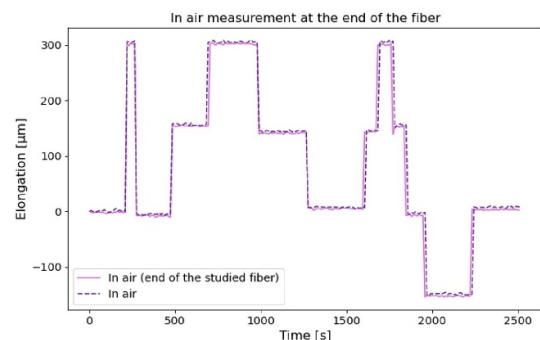
Figure 10. First results of the FSI ‘in-fiber’ measurements. Each portion has been tested, from top to bottom: small portion, medium portion, long portion and in air measurement done with the end of the studied fiber. The smallest portion studied was subject to sag when decreasing the distance between the platform and the reference, resulting in a decrease of the distance in air but not of the distance measured in fiber.
