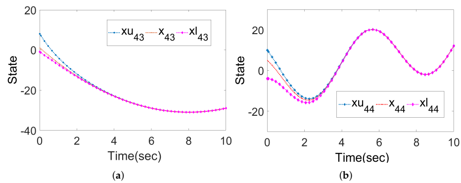
Figure 4. Evolutions of velocity of original system and DIO at the first joint (a) and second joint (b) of fourth manipulator.
