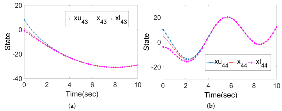
Figure 4. Evolutions of velocity of original system and DIO at the first joint (a) and second joint (b) of fourth manipulator.
