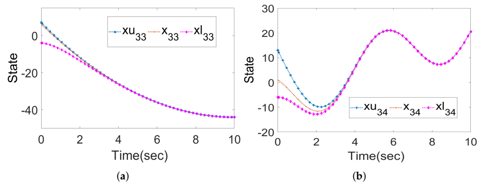
Figure 3. Evolutions of velocity of original system and DIO at the first joint (a) and second joint (b) of third manipulator.
