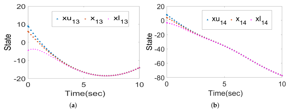
Figure 1. Evolutions of velocity of original system and DIO at the first joint (a) and second joint (b) of first manipulator.
