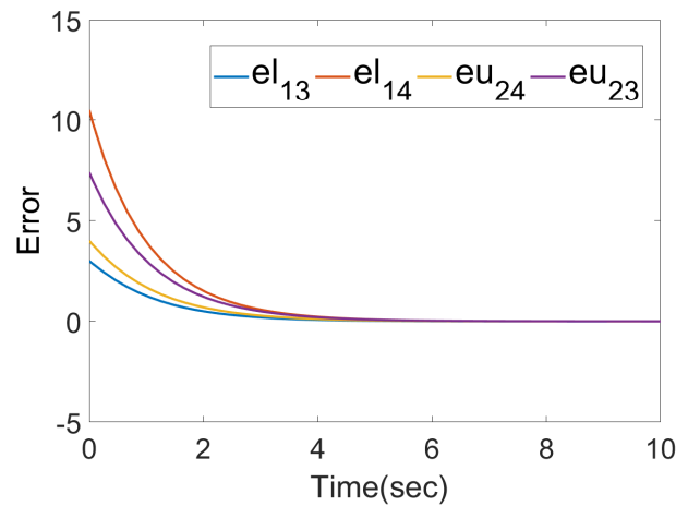
Figure 5. The error between the observer and the original system of the first manipulator.
