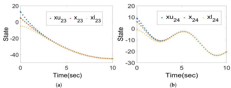
Figure 2. Evolutions of velocity of original system and DIO at the first joint (a) and second joint (b) of second manipulator.
