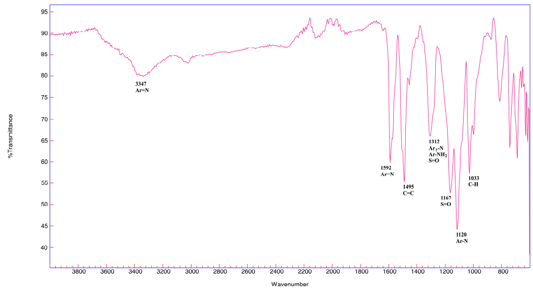
Figure 18. FTIR spectrum of Alkali blue 4B 9.
