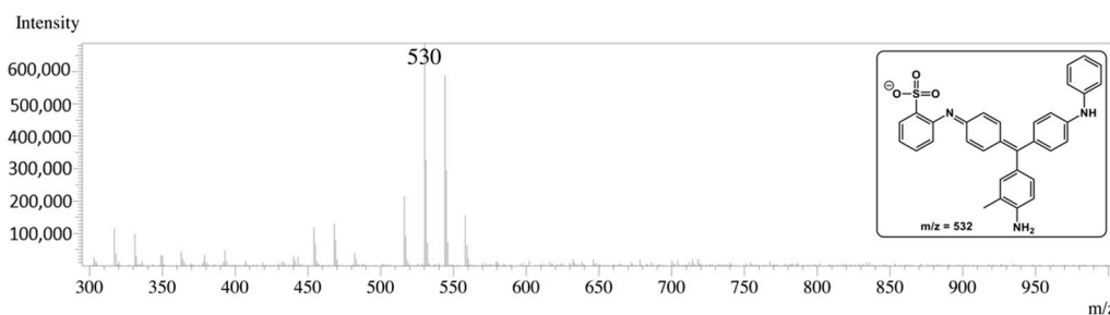
Figure 17. ESI-MS spectrum of Alkali blue 4B 9.
