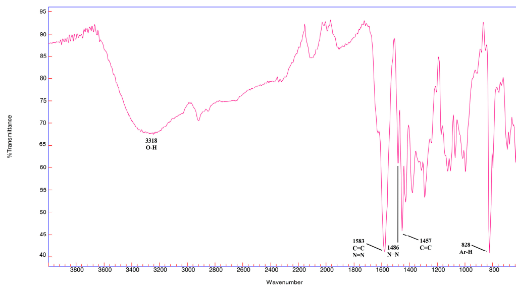
Figure 12. FTIR spectrum of Chrysamine G 3.
