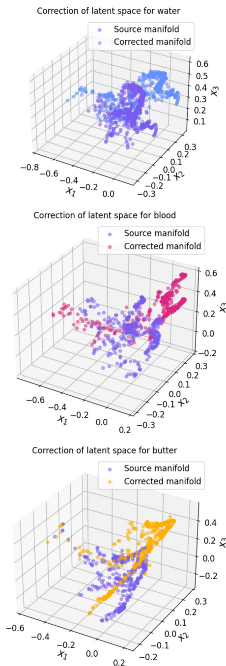
Fig. 3 Representation of the correction of the latent manifold of the position. The latent representation evolves to match the features of the new liquid
