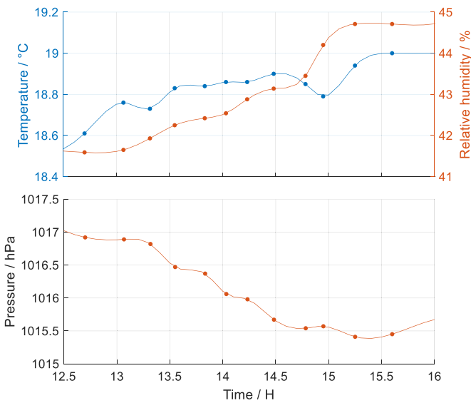
Figure 3. Environmental parameters recorded by a Vaisala PTU300 sensor and used by the multilateration system for air refractive index compensation. This sensor provides the temperature at \pm 0.2^\circ\text{C} , the pressure at \pm 0.25\text{ hPa} , and the relative humidity at \pm 1\% .
