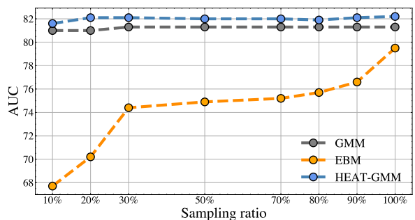
Figure 4. Impact on performances (AUC \uparrow on CIFAR-100) vs. the number of training data for GMM density, fully data-driven EBM, and HEAT. Our hybrid approach maintains strong performances in low-data regime, in contrast to the fully data-driven EBM.
