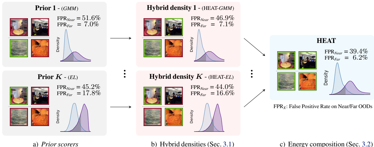
Figure 1. Illustration of our HEAT model. HEAT leverages a) K prior density estimators, such as GMM or EL, and overcomes their modeling biases by learning a residual term with an EBM b) leading to more accurate OOD scorers, e.g. HEAT-GMM or HEAT-EL. The second contribution is to combine the different refined scorers using an EBM energy composition function. The final HEAT prediction c) can thus leverage the strengths of the different OOD scorers, and be effective for both far and near-OOD detection.
