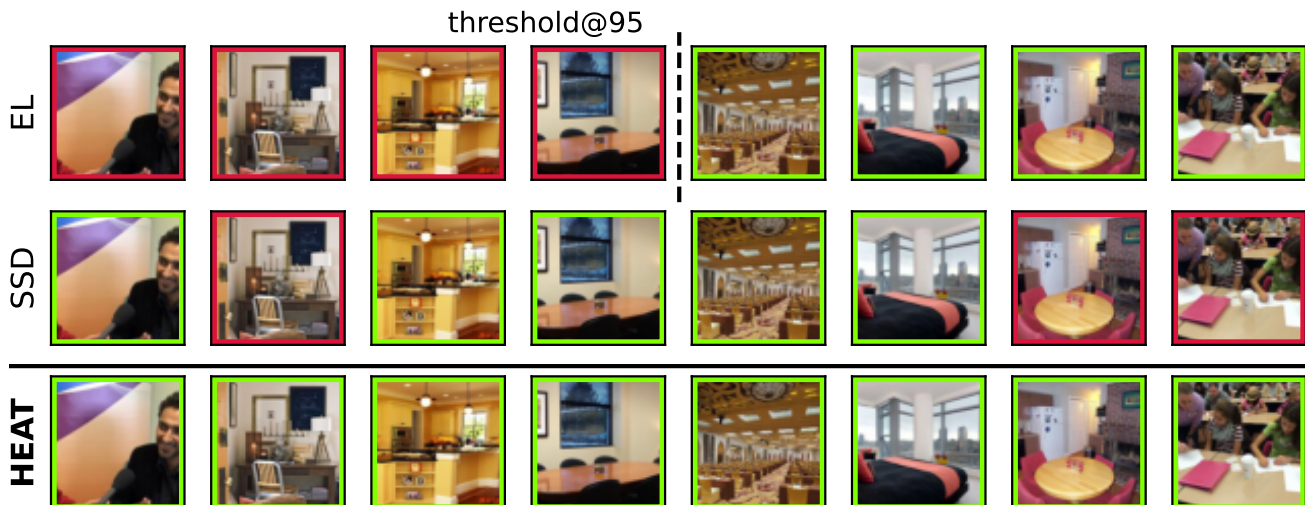
Figure 5. Qualitative comparison of HEAT vs.EL (Liu et al., 2020) and SSD (Schwag et al., 2021). Samples in green are correctly detected as OOD (LSUN), samples in red are incorrectly predicted as ID (CIFAR-10).
