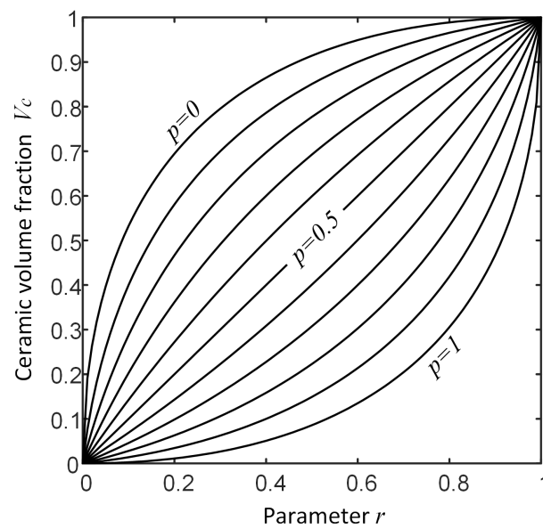
Figure 8. Ceramic volume fraction as function of controlling parameters p and r related to Equation (39).
