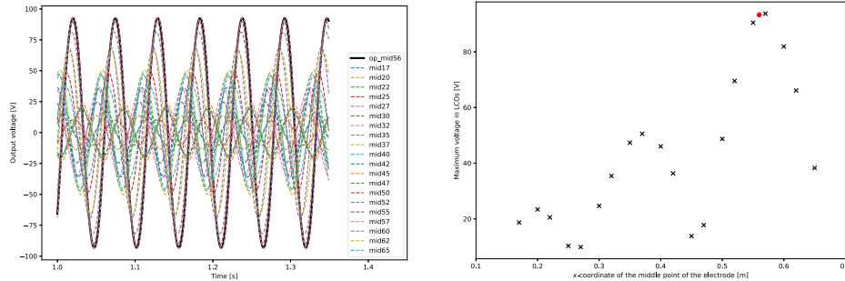
(j) v_\infty = 15.7 \text{ ms}^{-1} , \rho = 21.1 \text{ kgm}^{-3}
