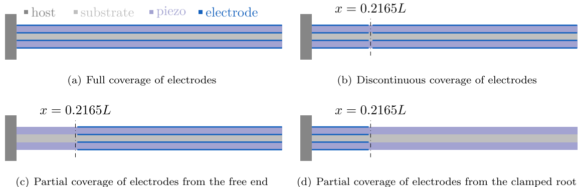
Fig. 2. Different electrode configurations. The last three figures, which take a PEH vibrating in the second mode as an example, illustrate the methods in literature to avoid charge cancellation.
