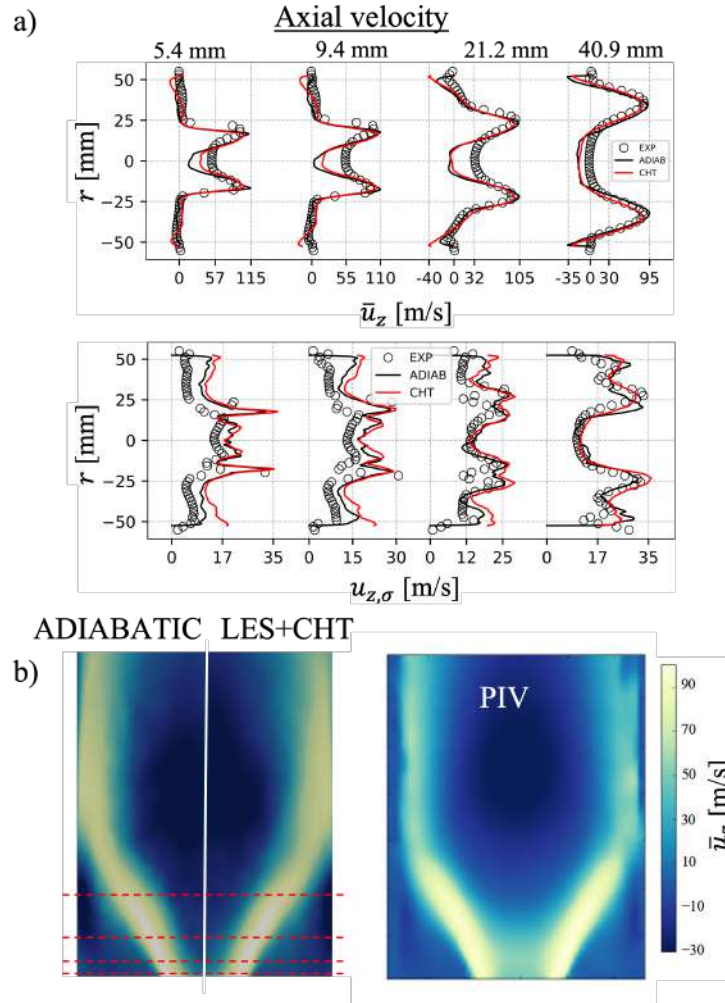
Figure 12: a) Axial velocity ( \bar{u}_z ) and its root mean square ( u_{z,\sigma} ) profiles at different streamwise positions inside the combustion chamber; b) comparison of the mean axial velocity contours calculated with AVBP and experimentally via PIV [63, 30].
