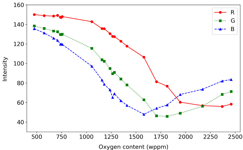
Fig. 8. Average values of Red (R), Green (G) and Blue (B) channels in the powder bed scans of oxidized powders in function of the oxygen content. (For interpretation of the references to color in this figure legend, the reader is referred to the web version of this article.)
