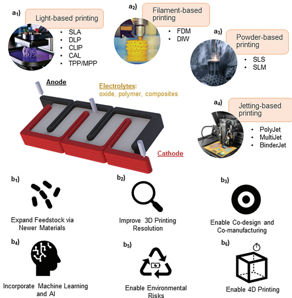
Figure 1. Additive manufacturing (AM) techniques for batteries, including a 1 ) light-based printing, a 2 ) filament-based printing, a 3 ) powder-based printing, and a 4 ) jetting-based printing, depicted with their respective subtypes. The schematic also illustrates future advancements to b 1 ) expand the feedstock of printers via new materials, b 2 ) improve the printing resolution, (b 3 ) adopt co-design and co-manufacturing methods, b 4 ) incorporate machine learning (ML) and artificial intelligence (AI) for optimized in-situ fabrication methods, b 5 ) navigate around the risks through implementing recycling methods for batteries, and b 6 ) enable 4D printing of energy storage devices.
