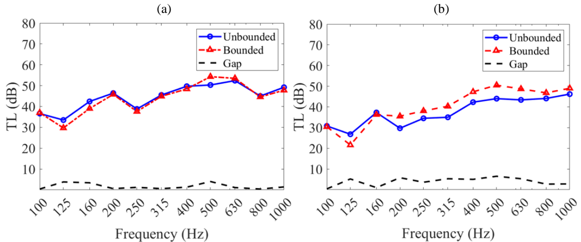
Fig. 16. Impact of position of the sound insulation material (melamine foam and heavy masses) on numerically computed Sound Transmission Loss (dB) for Isolated roller shutter boxes: (a) retracted and (b) extended
