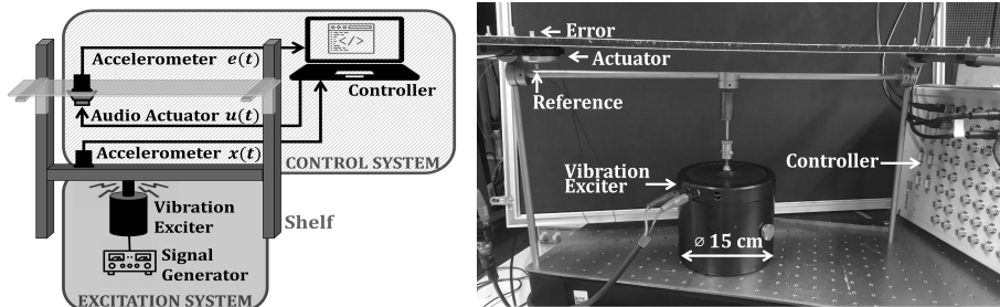
Fig. 5 Drawing (left) and photo (right) of the test bench used during experiments
