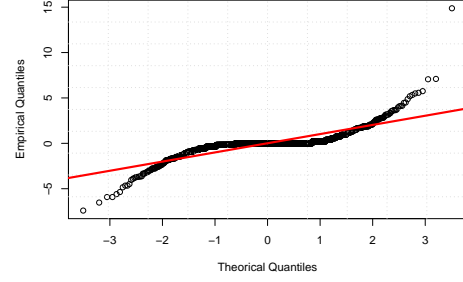
(b) Renault return series. QQ-Plot
