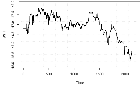
(a) Renault S.A., real
