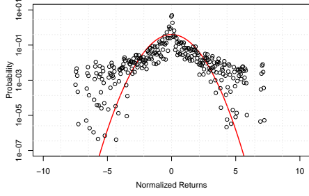
(a) Renault return series. Fat Tails (Normalized Returns)
