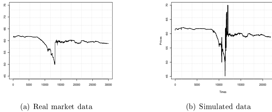
FIGURE 3 – Vinci equity on November 22, 2016. Left panel presents the actual price dynamics, right panel presents the would-be price dynamics without circuit breaker as simulated using ATOM.
