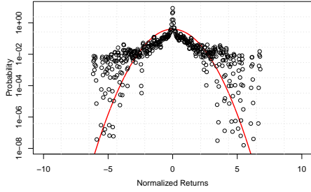
(c) Unconstrained ATOM ZIT. Fat Tails (Normalized Returns)
