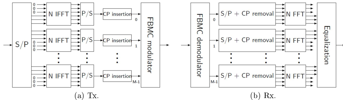
Figure 3.2: FFT-FBMC transceiver.
