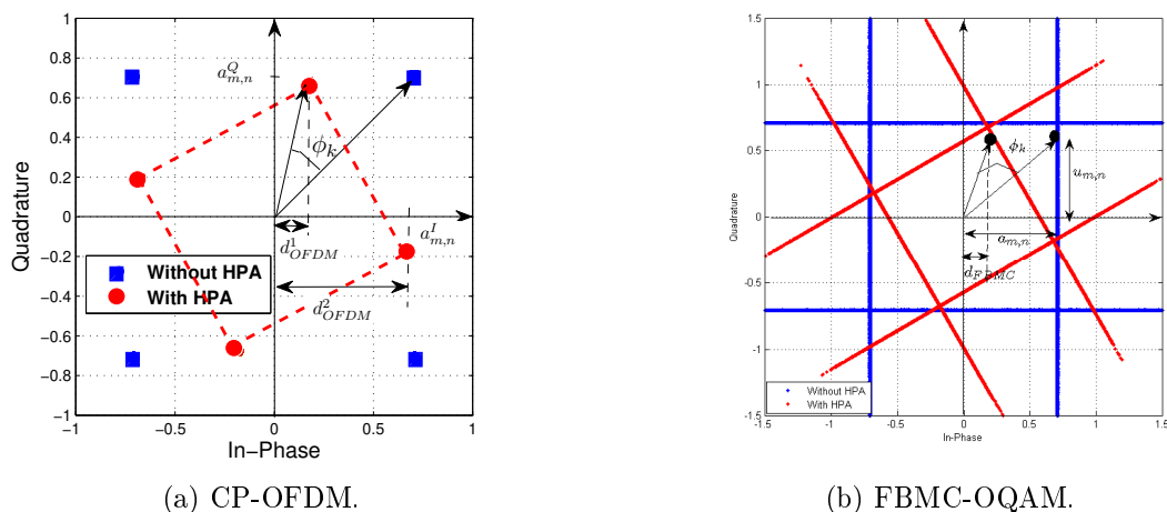
Figure 4.4: Example of 4QAM constellation before and after PA.
